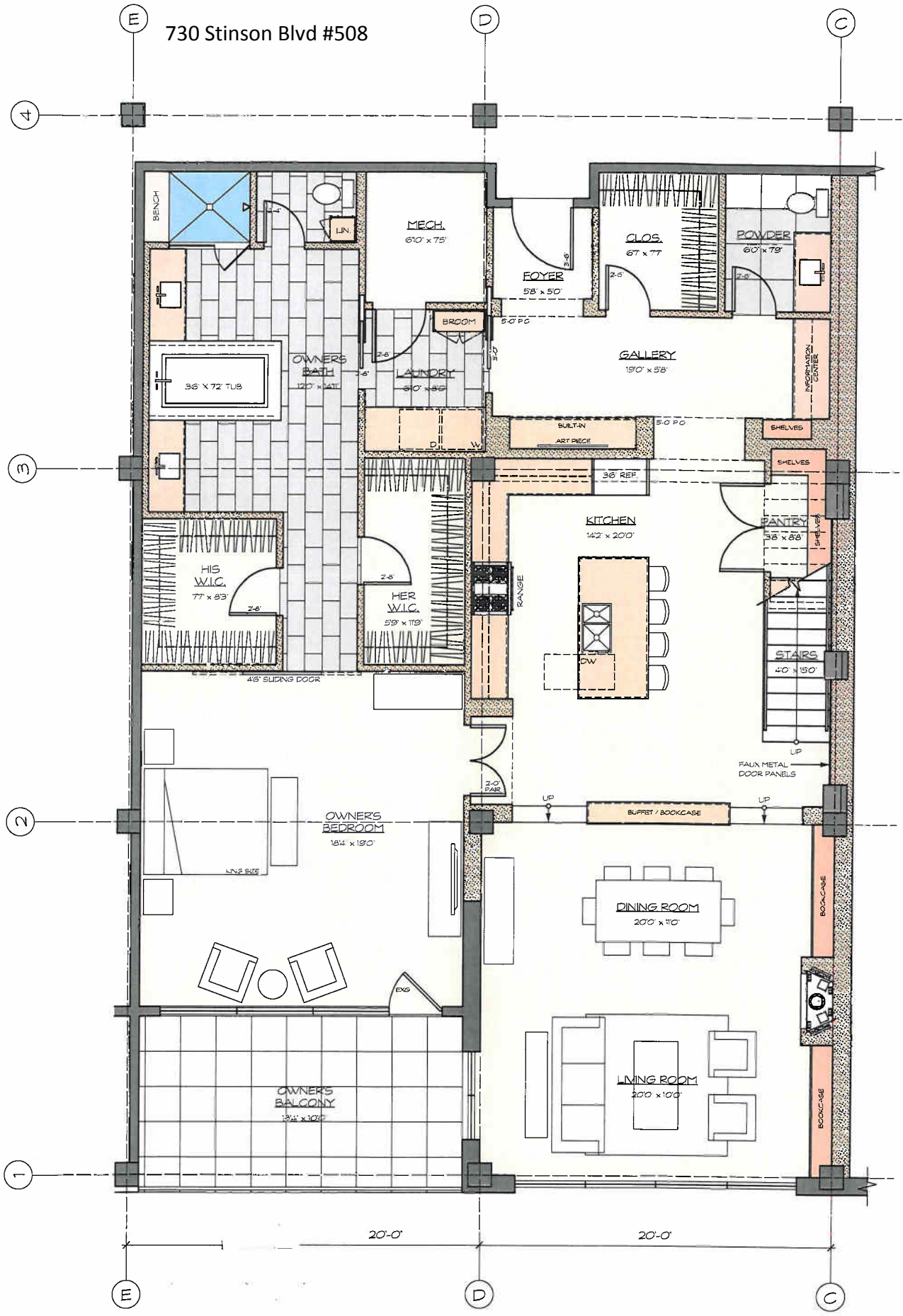
PROPOSED MAIN FLOOR PLAN - UNIT "A"
