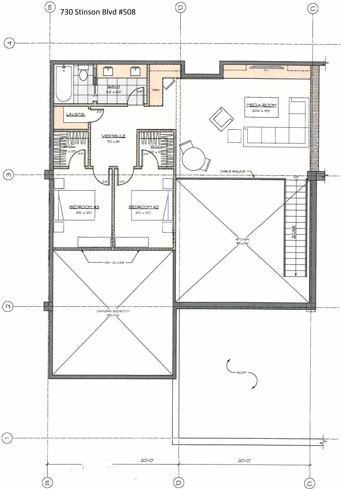
PROPOSED UPPER FLOOR PLAN - UNIT "A"
